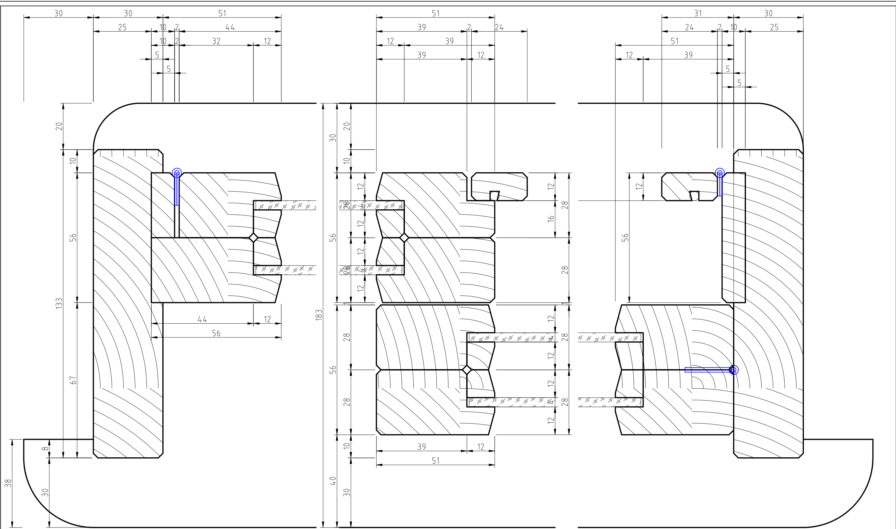
Shed Window Frame Side View M 1:1 Andreas Junius
